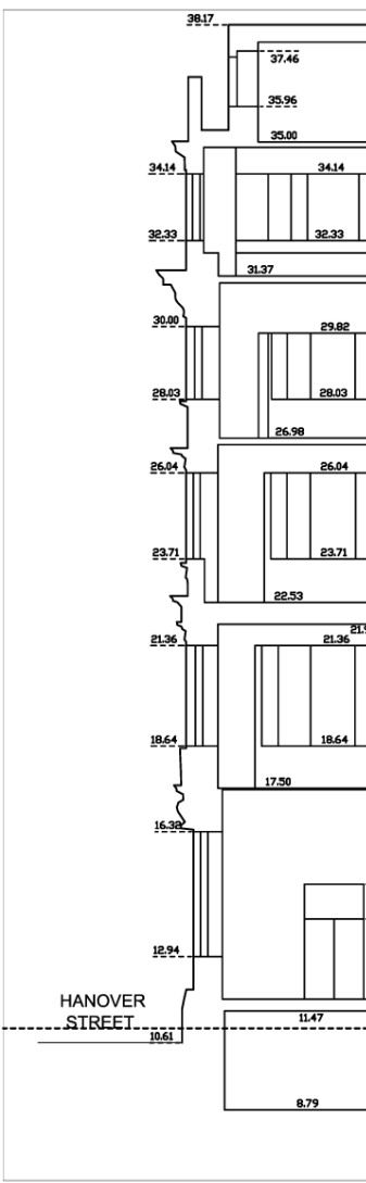
SECTION THROUGH WALL TO HANOVER STREET
